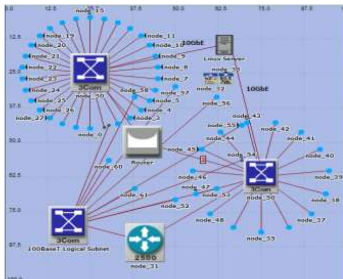
Fig:-Simulation setup for high speed optical communication through 100BaseT Ethernet.
